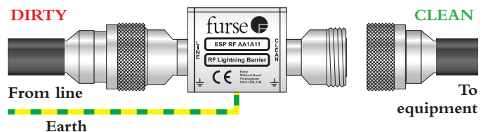
ESP RF AA1A11 with 7/16 DIN female connectors installed in series.
