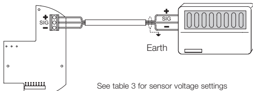
Diagram 9: Xgard Type 3 electrical connections
