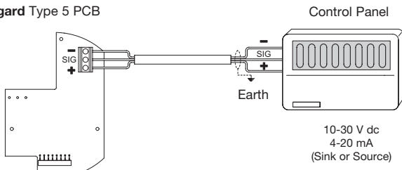
Diagram 13: Xgard Type 5 electrical connections
