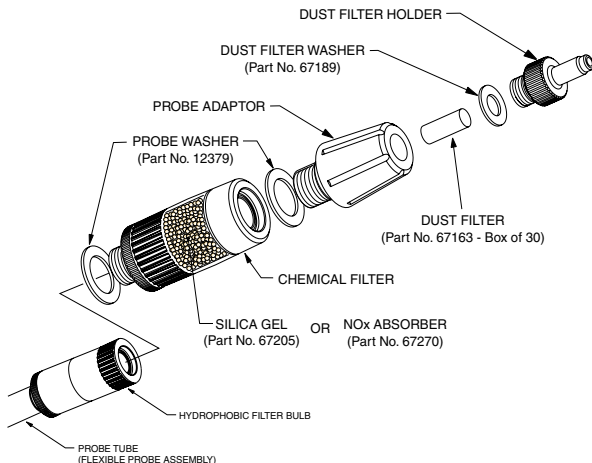
Fig. 13.3 Filter Removal
