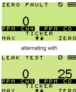
Fig. 4.1 Sensor Check
