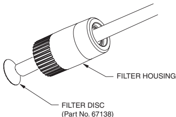
Fig. 13.5 Housing Filter Removal
