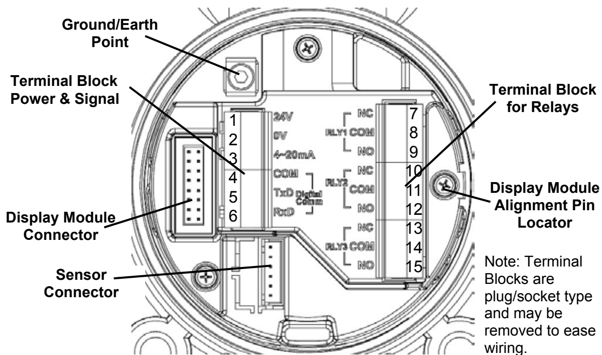
Diagram 7: Terminal module
