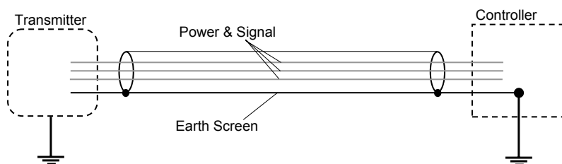
Diagram 10: System grounding
