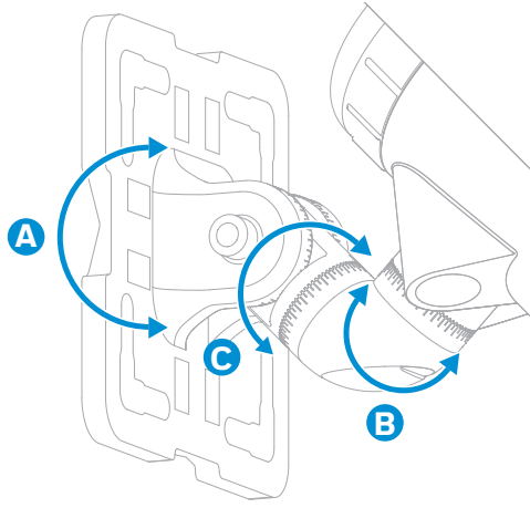
Figure 6. Adjustment ranges
