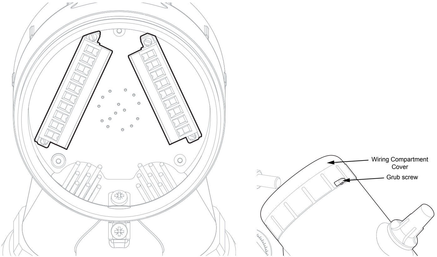
Figure 18. PCB Terminals
