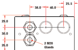
Dimensions of piped exhaust docking station
