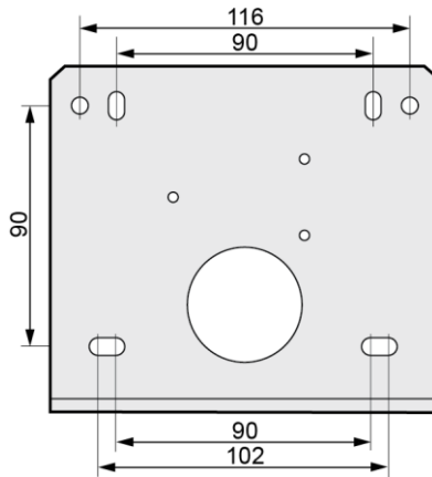
Figure 3: drilling diagram for wall mounting (view of the side flattened onto the ceiling).
