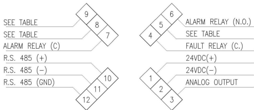
Figure 6: Wiring Terminals
