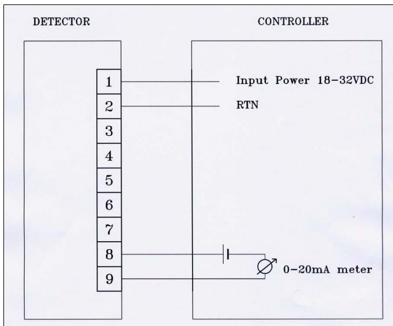
Figure 8: 0-20mA Wiring Option 1 (Sink 4-Wire) - Default
