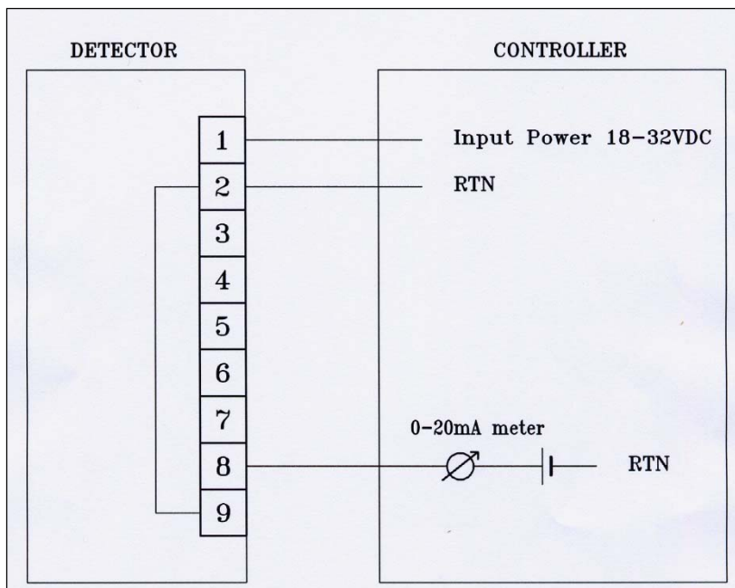
Figure 10: 0-20mA Wiring Option 1 (Non-isolated Sink 3-Wire)
