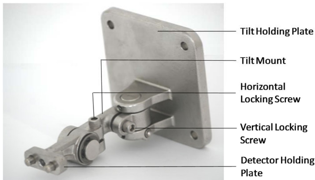
Figure 3: Tilt Mount Assembly
