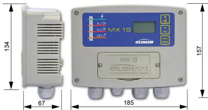
Figure 4: Dimensions of the controller
