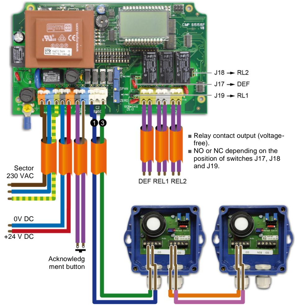
Figure 5: MX 15 controller and two OLCT 10 sensors for detection of the same toxic gas (maximum 5 sensors).
