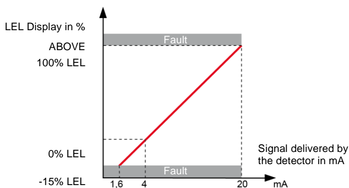
Figure 9: Configuration transfer curve 0 to 100 % LEL
