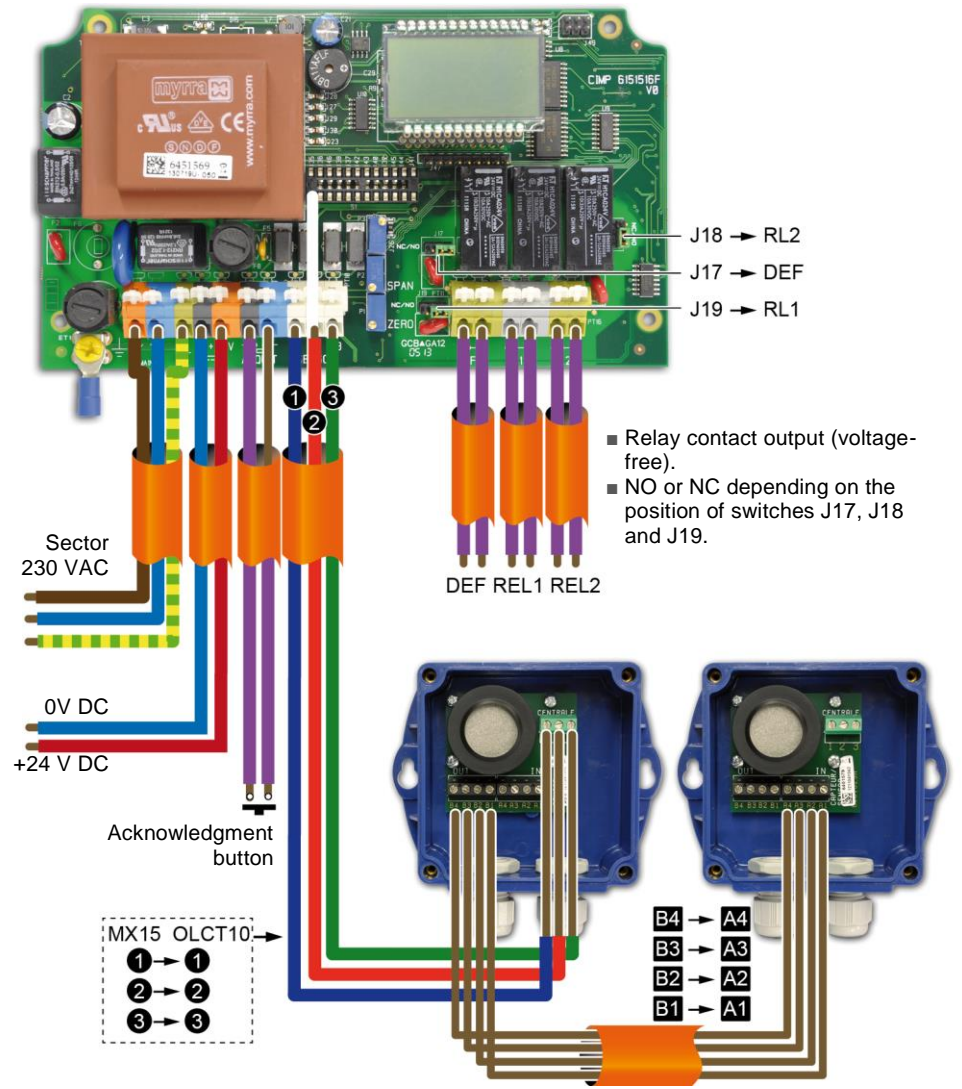
Figure 6: MX 15 controller and two type OLC 10 TWIN sensors.
