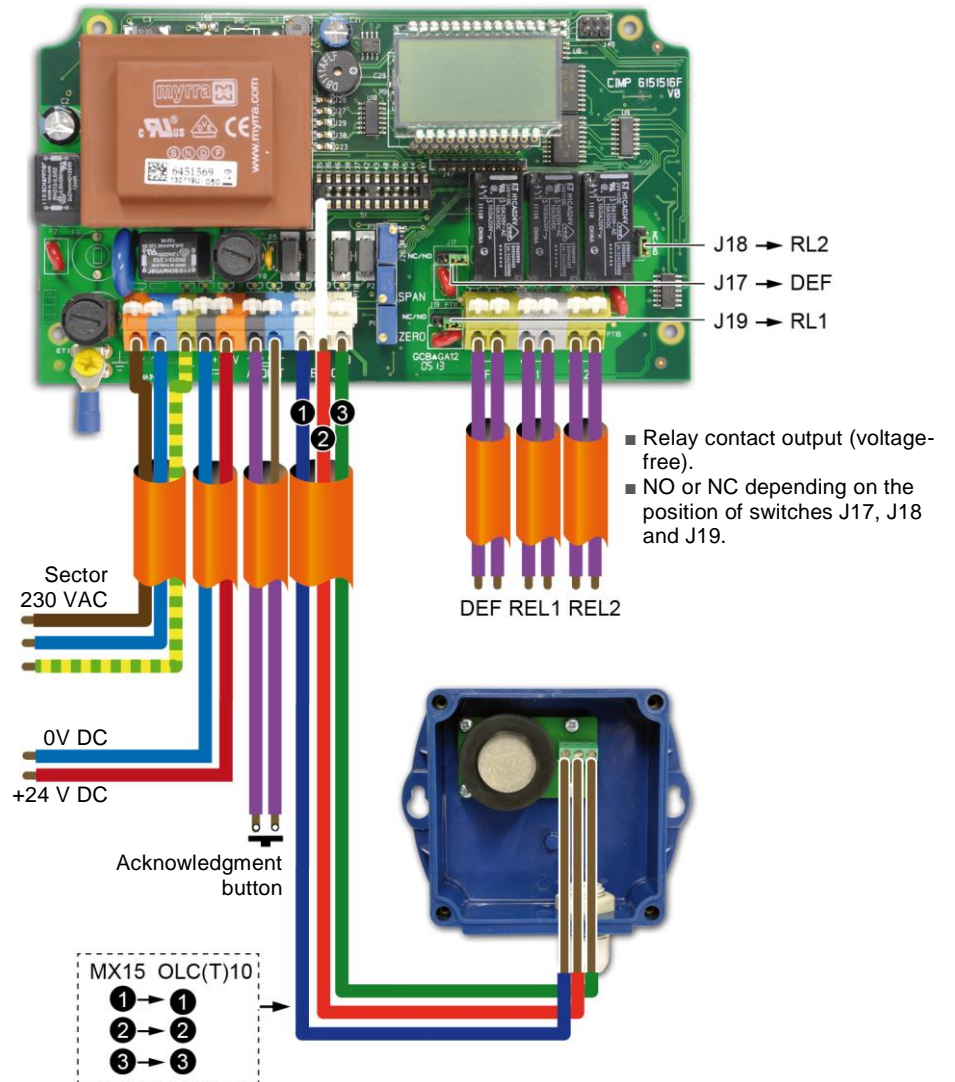
Figure 7: MX 15 controller and a 3-active wire EXPLO or TOXIC sensor.
